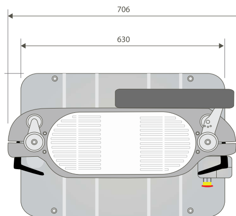
E3000 dimensions: plan view
